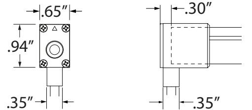
TRACE RGBW LEAD - BOTTOM Horizontal Bottom Lead Entry 5' Power Lead Cable with End Cap
