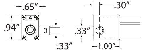
TRACE RGBW LEAD - SIDE Horizontal Side Lead Entry 5' Power Lead Cable with End Cap
